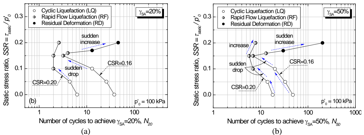
Figure 7. Relationship between static stress ratio and number of cycles to cause: (a) Single amplitude shear strain of 20%; (b) Single amplitude shear strain of 50%
