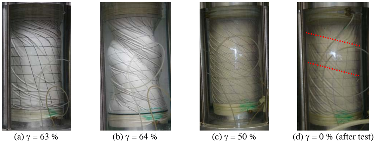
Photo 1. Typical specimen deformation: (a) Reversal tests 16-10; (b) Intermediate test 16-16; (c) Non-reversal tests 16-20; and (d) Spiral shear band for non-reversal tests 16-20.
