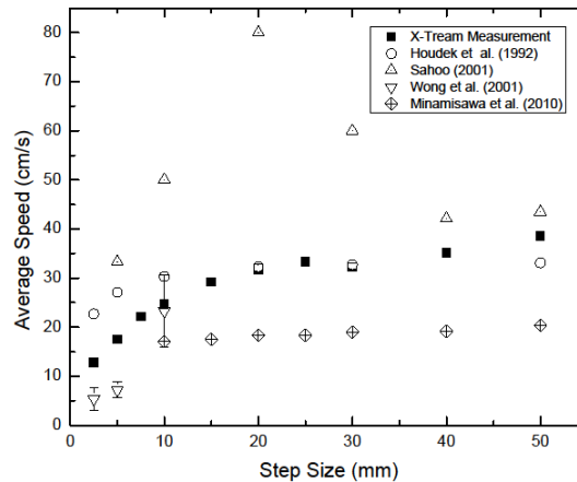
425 Figure 14 - Average transit speed measured using X-Tream System (black). Results extracted from the literature are shown for comparison.
