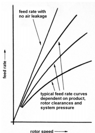
Figure 1 Typical feed rate characteristics [1]
