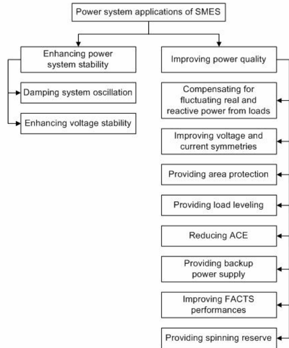
Fig. 7. Classification of SMES applications to power systems
