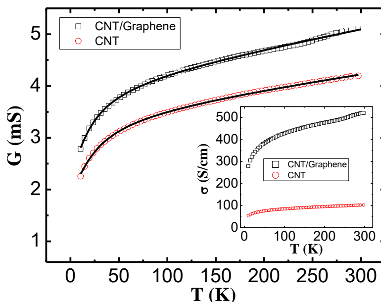
Figure 4. The temperature dependence of conductance G (T) of the CNT yarn and CNT/graphene yarn. The solid curves show the two shell model fitting to experimental data. Inset: Conductivity as a function of temperature for both samples.
