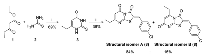
Scheme 1 Reagents and conditions: (i) NaOEt, C 2 H 5 OH, 6 h, reflux; (ii) ClCH 2 COOH, anhydrous CH 3 COONa, (CH 3 CO) 2 , CH 3 COOH, 4-chlorobenzaldehyde, reflux, 4 h.
