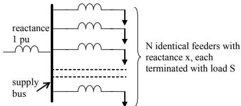
Fig. 3 – System with N homogenous feeders
