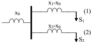
Fig. 2 – Two feeder system
