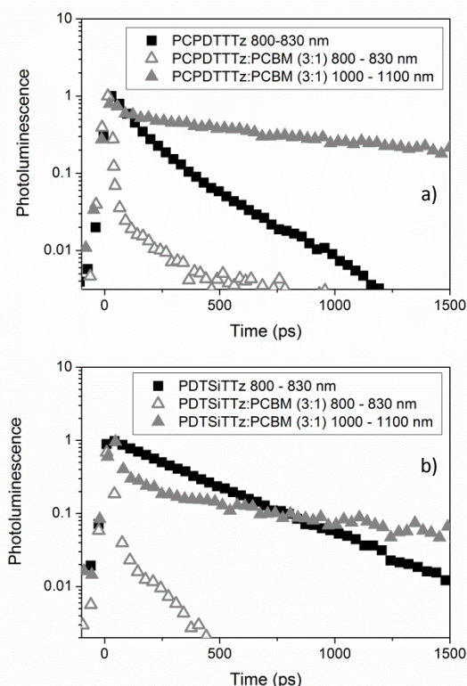
Figure 6. The photoluminescence decays with time for pristine PCPDTTz (a) and PDTSiTTz (b) and their 3:1 blends with PCBM, on encapsulated quartz and measured in the spectral ranges 800-830 nm (polymer emission) and 1000-1100nm (CT state emission).
