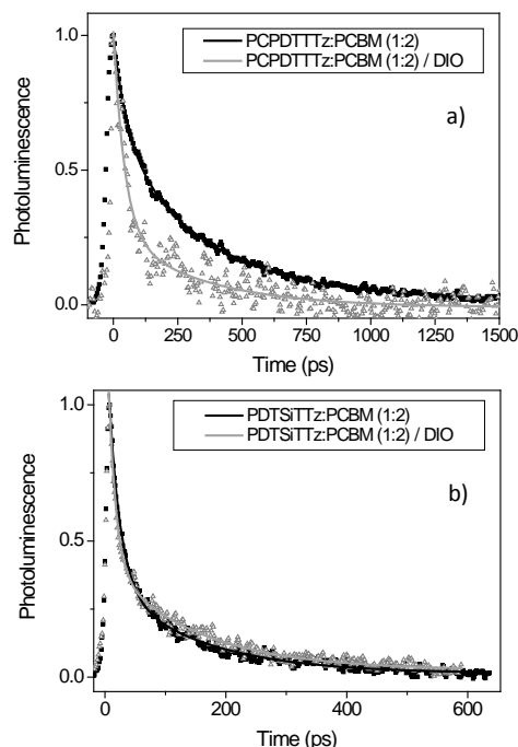
Figure 7. The photoluminescence decays for PCPDTTz:PCBM (a) and PDTSiTTz:PCBM (b) 1:2 blends, on encapsulated quartz and measured in the spectral range of 1000-1100 nm, showing the effect of the DIO.
