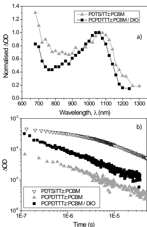
Figure 4. Transient absorption spectrum of PDTSiTTz:PCBM and PCPDTTTz:PCBM (1:2, with DIO) blend films (a) and a comparison of the charge carrier dynamics for PCPDTTTz:PCBM and PDTSiTTz:PCBM (1:2) blend films with and without DIO, measured using 3 \mu\text{Jcm}^{-2} 532 nm excitation and a 1000 nm probe (b).
