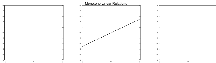
Fig. 5 The three possible forms of a monotone linear relation on \mathbb{R} .
