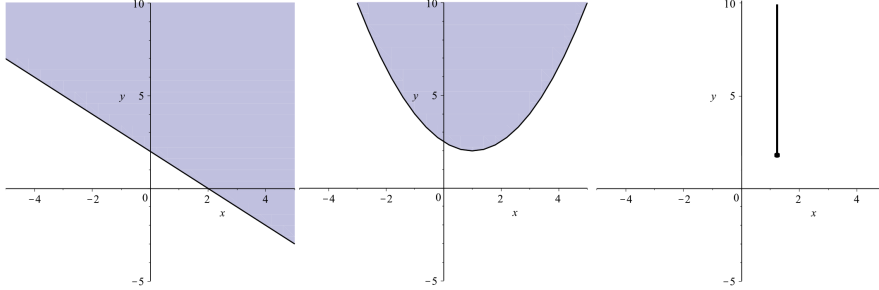
Fig. 1 The three possible general forms of the epigraph of f(x) .
