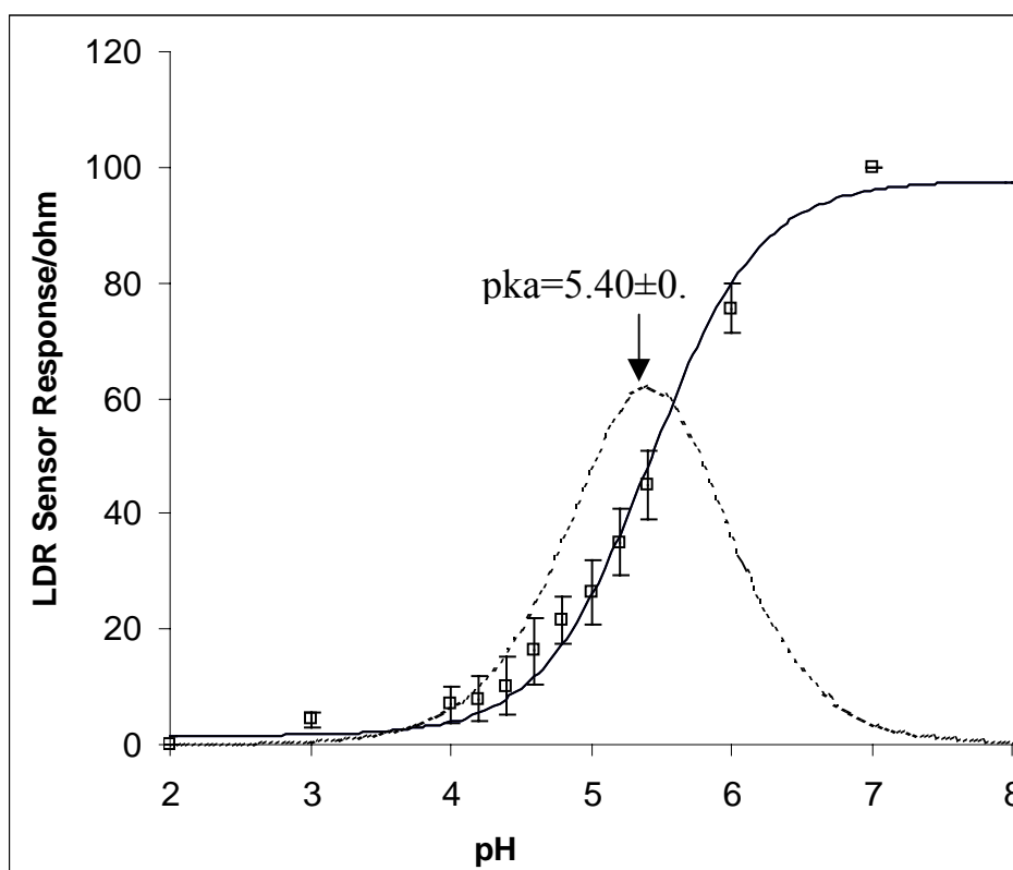
Figure 4. Response curve obtained from LDR sensor. The solid sigmoidal line is the best-fit line obtained by using MicroSoft Excel Solver. The Error bars represent standard deviations of three repeats. The Gaussian curve is the first derivative of the best-fit line to obtain the pKa value for the dye.
