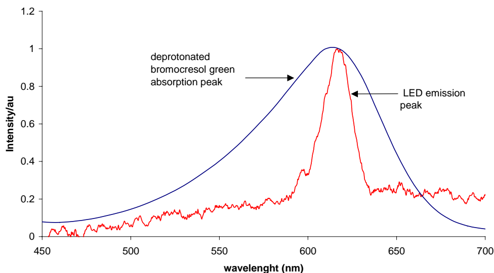
Figure 1. Absorption spectrum of bromocresol green overlaps perfectly with emission spectrum of the LED light source to achieve optimal sensor sensitivity.
