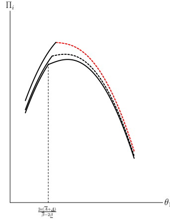
Figure 2: Profit functions for different values of the A -side profits
