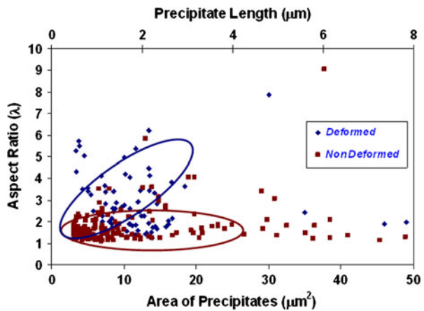
Fig. 6—A comparison between the aspect ratios of precipitates in deformed (at 1273 K (1000 °C)) and nondeformed areas of Gleeble samples.
