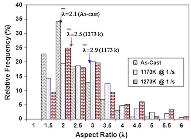
Fig. 7—Relative frequency for aspect ratio of precipitates deformed at different temperatures ( \bar{\lambda} in each group is the mean value of at least 300 precipitates).
