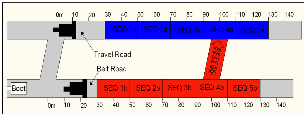
Figure 5 - Super panel sequence plan
