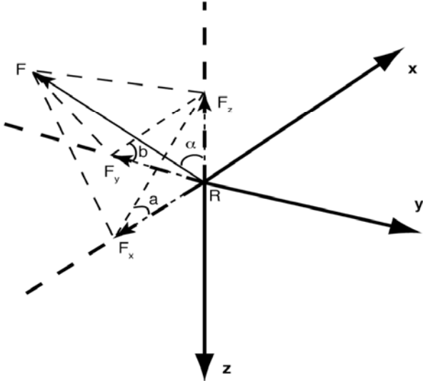
Figure 5 Thrust vectors
