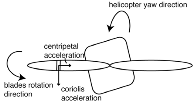
Figure 7 Centripetal and coriolis acceleration – top view
