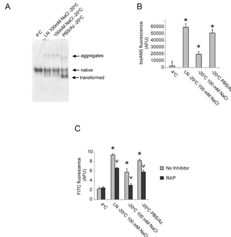
Fig 4. The effect of storage at -20°C on the ability of \alpha_2 M to bind to SH-SY5Y cells. (A) Image of a native PAGE (3–8% Tris-acetate) gel showing \alpha_2 M stored in 20 mM sodium phosphate buffer, pH 7.4 containing 100 mM NaCl or in PBS/Az (4°C or -20°C, 10 days). LN indicates that the sample was rapidly frozen in liquid nitrogen prior to storage at -20°C. (B) Corresponding bisANS fluorescence measurements for \alpha_2 M stored as described in (A). The results shown are the mean values of bisANS fluorescence ( n = 3 \pm SD ) in AFU. (C) Flow cytometry analysis showing the binding of \alpha_2 M preparations stored as described in (A) to SH-SY5Y cells. The results shown are the composite geometric mean values of FITC fluorescence for 5000 viable cells ( n = 3 \pm SD ) in AFU and are adjusted for background fluorescence. * Denotes significant increases in cell surface binding of \alpha_2 M stored at -20°C compared to a batch matched sample stored at 4°C. v Denotes significant decreases in cell surface binding of \alpha_2 M as a result of pre-incubation of the cells with RAP.
