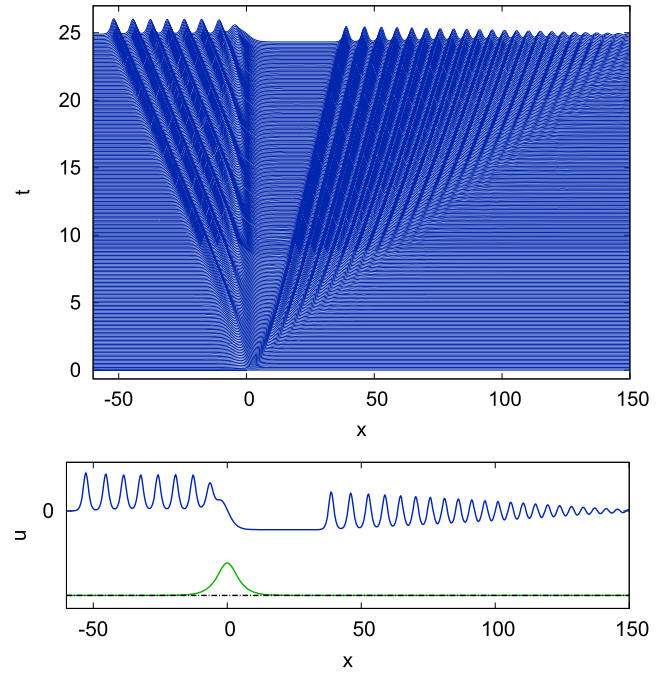
FIG. 1. Solution of the forced eKdV equation (1). A perspective view in the x-t plane (top) and the surface profile u and bathymetry G versus x at t = 25 (bottom) are shown. The numerical solution of (1) with the initial condition u = 0 is shown. The parameters are \alpha = 0.15 and \Delta = 0 .
