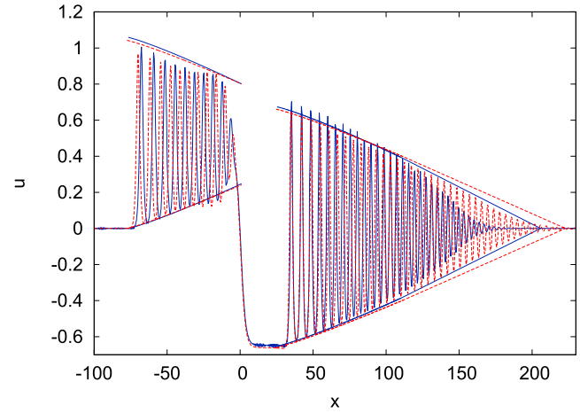
FIG. 7. Solution u versus x at t = 30 for surface water waves. Numerical solutions of the forced eKdV equation (blue solid line) and the forced KdV equation (red dashed line) are compared. The other parameters are \alpha = 0.15 and \Delta = -0.5 . Also shown are the wave envelopes for the upstream and downstream undular bores given by the eKdV (blue solid line) and KdV modulation theories (red dashed line).
