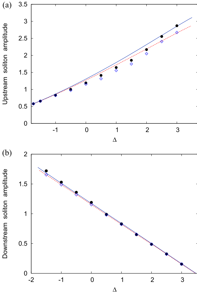
FIG. 4. (a) The upstream and (b) downstream solitary wave amplitudes versus the detuning parameter \Delta for surface water waves. The eKdV (blue solid lines) and KdV (red dashed lines) modulation theories and eKdV ( \bullet ) and KdV ( \diamond ) numerical solutions are compared. The other parameter is \alpha = 0.15 .
