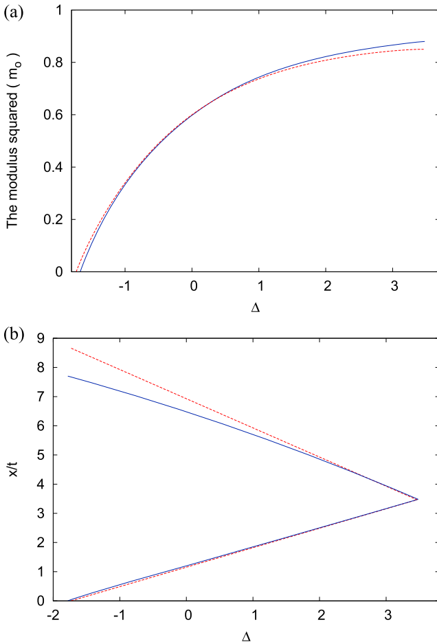
FIG. 3. (a) The modulus squared m_0 and (b) the leading and trailing edges of the downstream undular bore, \frac{x}{t} , versus the detuning parameter \Delta for surface water waves. The eKdV (blue solid lines) and KdV (red dashed lines) modulation theories are compared. The other parameter is \alpha = 0.15 .
