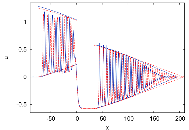
FIG. 5. The solution u versus x at t = 30 , for surface water waves. Numerical solutions of the forced eKdV equation (blue solid line) and the forced KdV equation (red dashed line) are compared. The other parameters are \alpha = 0.15 and \Delta = 0 . Also shown are the wave envelopes for the upstream and downstream undular bores for eKdV (blue solid line) and KdV (red dashed line) modulation theories.
