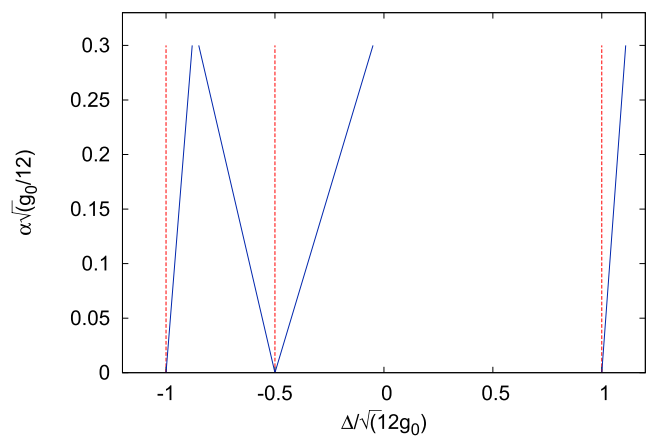
FIG. 2. The parameter ranges in the \Delta(12g_0)^{-\frac{1}{2}} versus \alpha(\frac{12}{g_0})^{\frac{1}{2}} plane for full and partial undular bores for surface water waves. The eKdV (blue solid lines) and KdV (red dashed lines) modulation theories are compared. Moving from left to right, the three sets of curves bound the subcritical limit of the bore, the transition between the partial and full bore, and the supercritical limit of the bore. For the middle set of curves, the eKdV downstream bore curve is on the left and the eKdV upstream bore curve is on the right.
