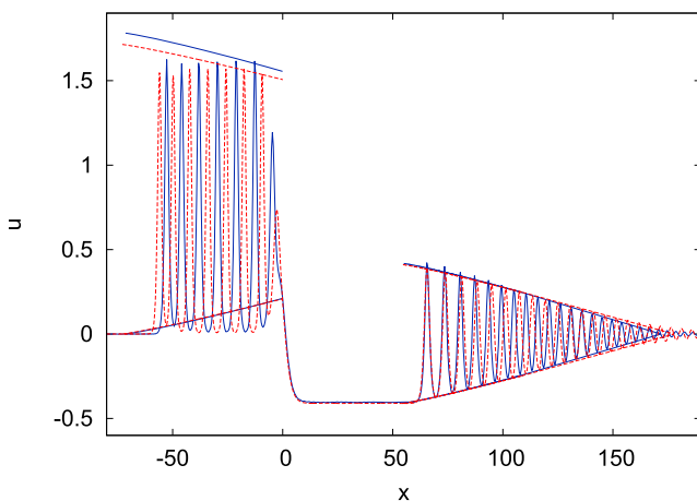
FIG. 6. Solution u versus x at t = 30 for surface water waves. Numerical solutions of the forced eKdV equation (blue solid line) and the forced KdV equation (red dashed line) are compared. The other parameters are \alpha = 0.15 and \Delta = 1 . Also shown are the wave envelopes for the upstream and downstream undular bores given by eKdV (blue solid line) and KdV modulation theories (red dashed line).
