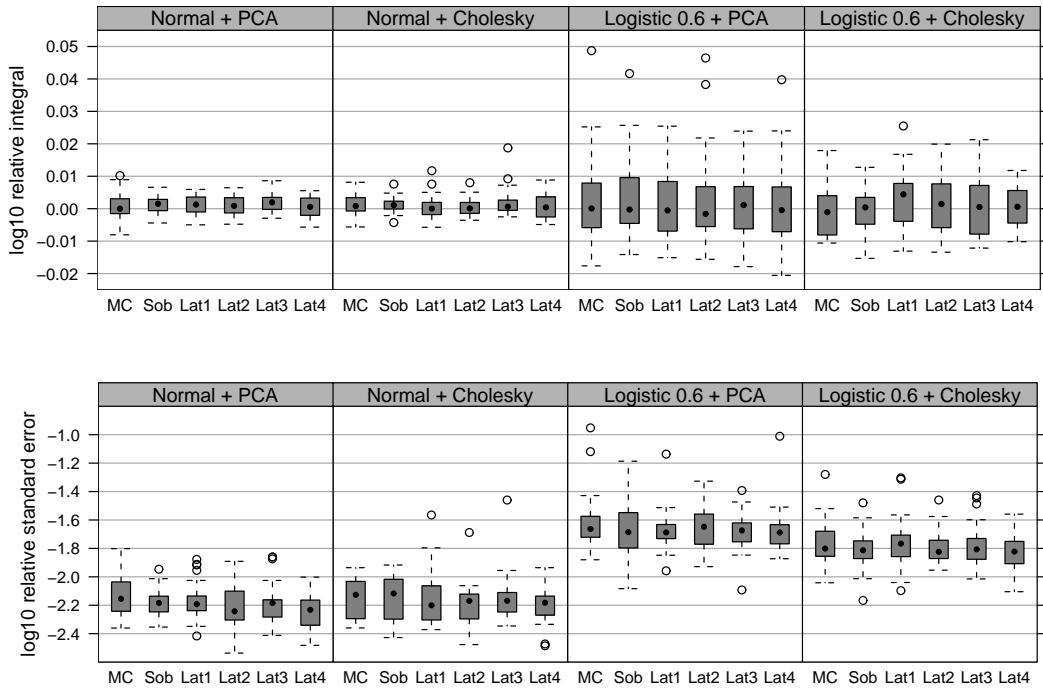
Figure 8: Example 1 with d = 200 . \log_{10} relative integrals and \log_{10} relative standard errors obtained from 30 repetitions based on 10 random shifts of 65536 points.
