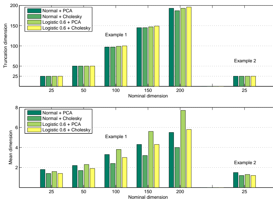
Figure 3: Effective dimensions of transformed integrands.
