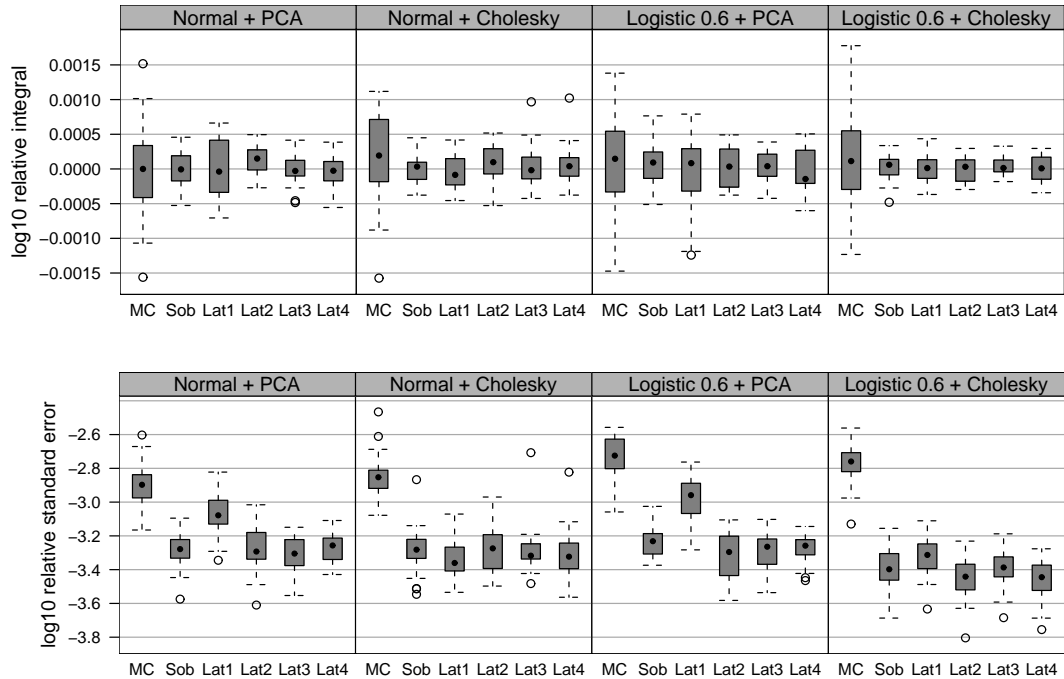
Figure 6: Example 1 with d = 25 . \log_{10} relative integrals and \log_{10} relative standard errors obtained from 30 repetitions based on 10 random shifts of 32768 points.
