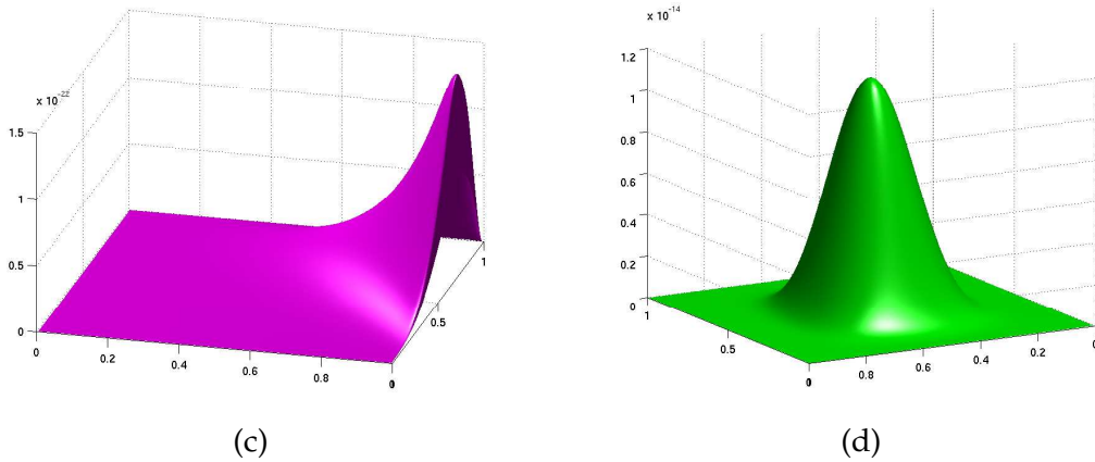
Figure 5: Two-dimensional projections of transformed integrand obtained (c) without centring and rescaling and (d) with centring but without rescaling.
