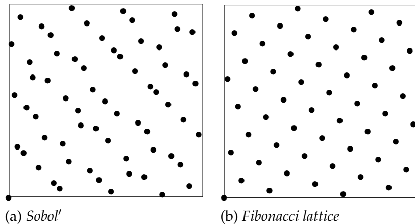
Figure 2: Digital net versus lattice rule.
