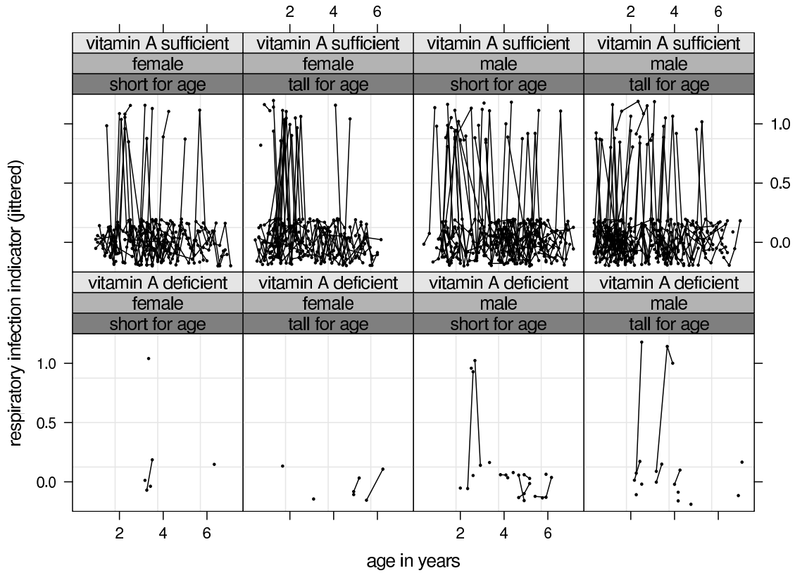
Figure 1: Respiratory infection indicator (0=absent, 1=present) versus age in years for a cohort of Indonesian children. Repeated measures on same child are connected by lines. Each panel corresponds to a different combination of three covariates: vitamin A nourishment, gender and height for age. The respiratory infection indicator has been jittered to enhance visualisation.
