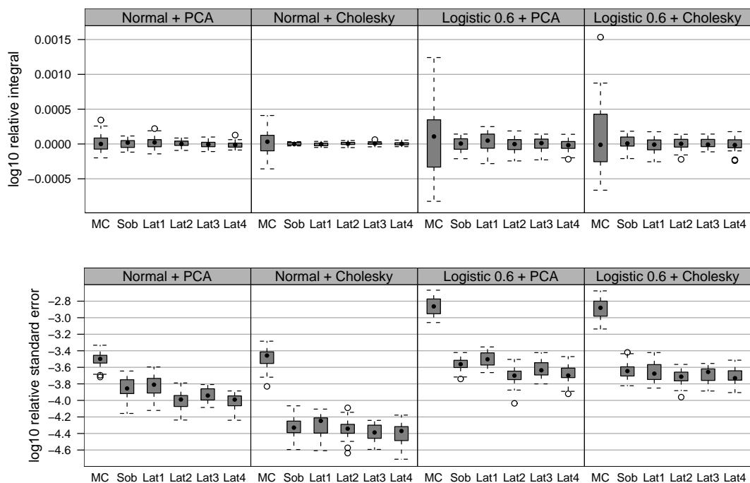
Figure 7: Example 2 ( d = 25 ). \log_{10} relative integrals and \log_{10} relative standard errors obtained from 30 repetitions based on 10 random shifts of 32768 points.
