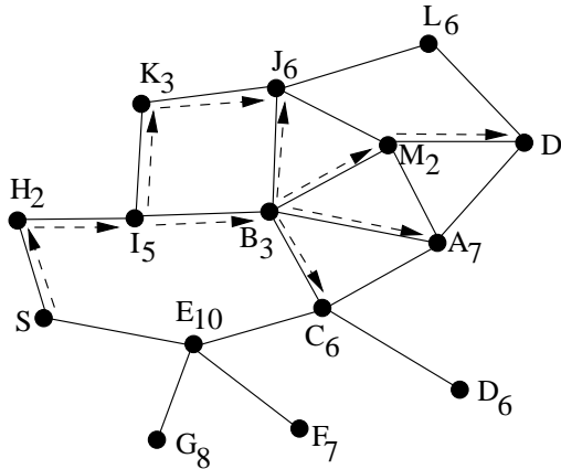
Fig. 2. Data packet fwb using FSF
