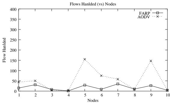
Fig. 10. TFN: 10 Nodes and 5 Flows
