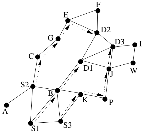
Fig. 2. Data packet fwb using FSF
