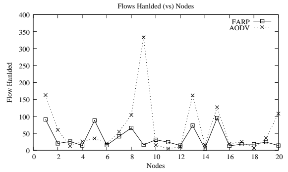
Fig. 11. TFN: 20 Nodes and 10 Flows
