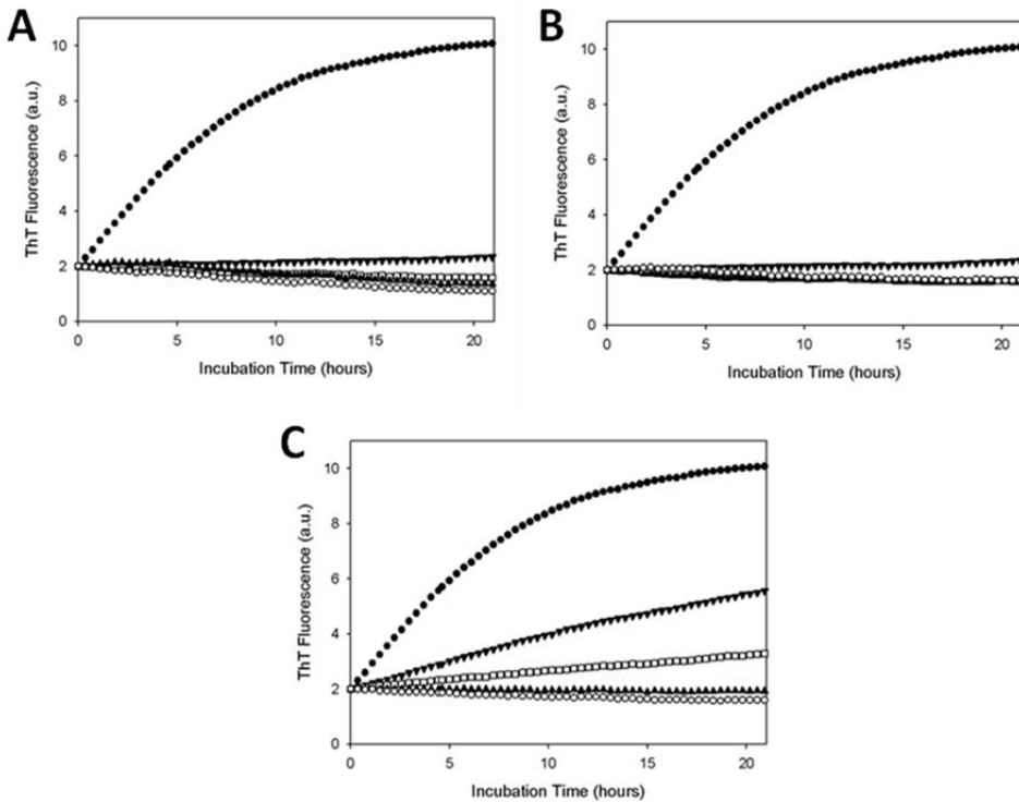
Figure 9. Chaperone activity of A) \alpha s -, B) \alpha s1 - and C) \alpha s2 -casein against amyloid forming RCM- \kappa -casein as determined by Thioflavin T (ThT) fluorescence. Ratios of chaperone:RCM- \kappa -casein equivalent to ~0.6:1, 1.25:1 and 2.5:1 (w:w) are represented by ▼, □ and ▲, respectively. Reprinted with permission from [17]. Copyright (2011) Elsevier Inc.
