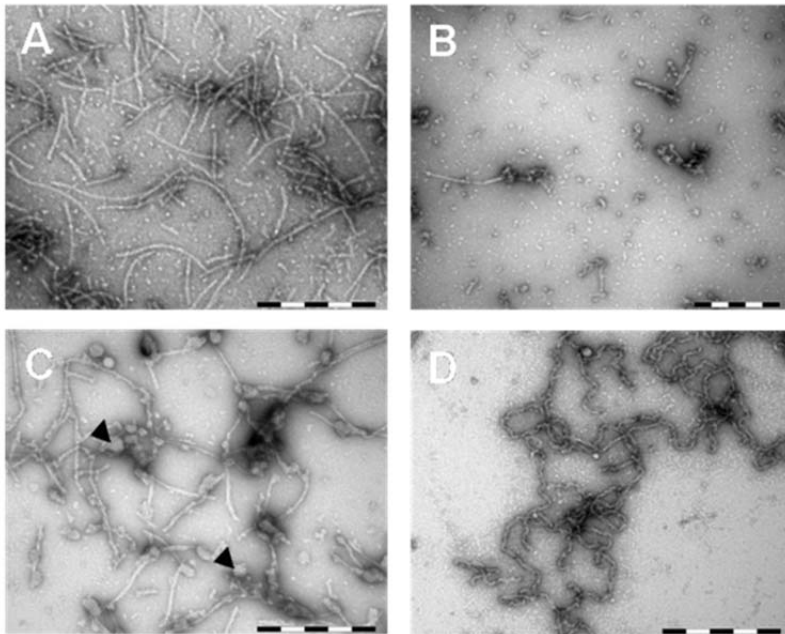
Figure 10. Electron micrographs of RCM- \kappa -casein incubated for 50 h at 37°C with and without \alpha_s -casein proteins. RCM- \kappa -casein incubated in the absence (A) or presence of \sim 1.0 mol:mol ratio (3.75 mg/mL) of either \alpha_{s1} -casein (B) or \alpha_{s2} -casein (C). \alpha_{s2} -Casein alone is also shown (D; 3.75 mg/mL). In (C), small, rounded aggregates are indicated by \blacktriangle . Scale bars represent 500 nm. Reprinted with permission from [17]. Copyright (2011) Elsevier Inc.
