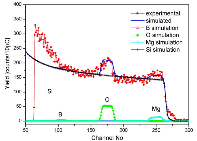
Fig. 2. RBS spectrum of MgB 2 film grown by PLD on Si (001) substrate and annealed in situ .
