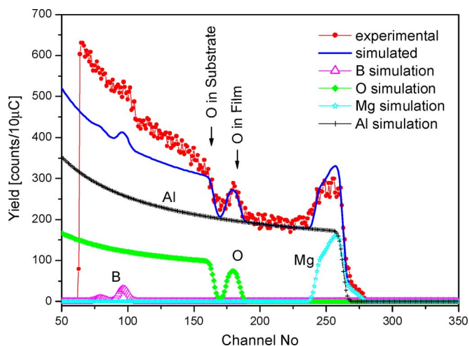
Fig. 3. RBS spectrum of an \text{MgB}_2 film grown by on-axis PLD on \text{Al}_2\text{O}_3 and annealed in situ .
