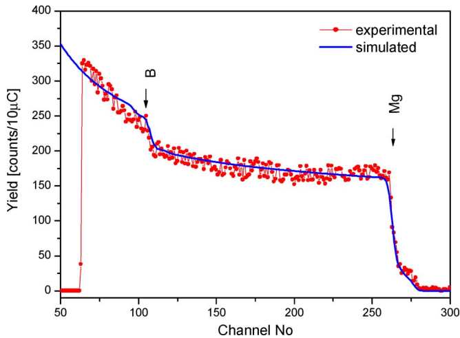
Fig. 1. RBS spectrum of the MgB 2 target.
