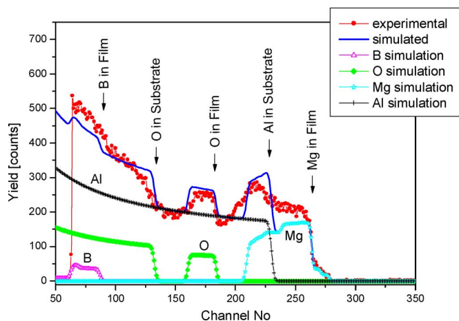
Fig. 4. RBS spectrum of an \text{MgB}_2 film grown by off-axis PLD on \text{Al}_2\text{O}_3 and annealed in situ .
