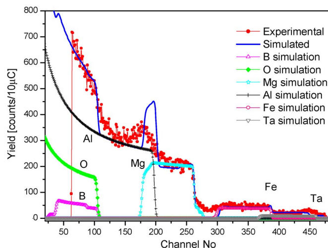
Fig. 5. RBS spectrum of an \text{MgB}_2 film deposited by PLD on \text{Al}_2\text{O}_3 and annealed ex situ .
