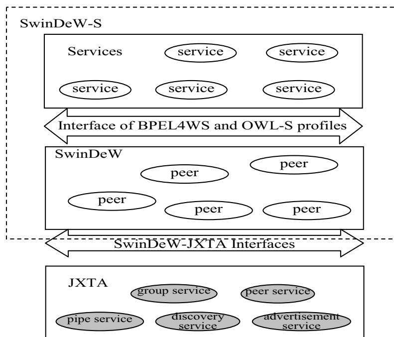
Figure 1: SwinDeW-S with Service Profile Support
