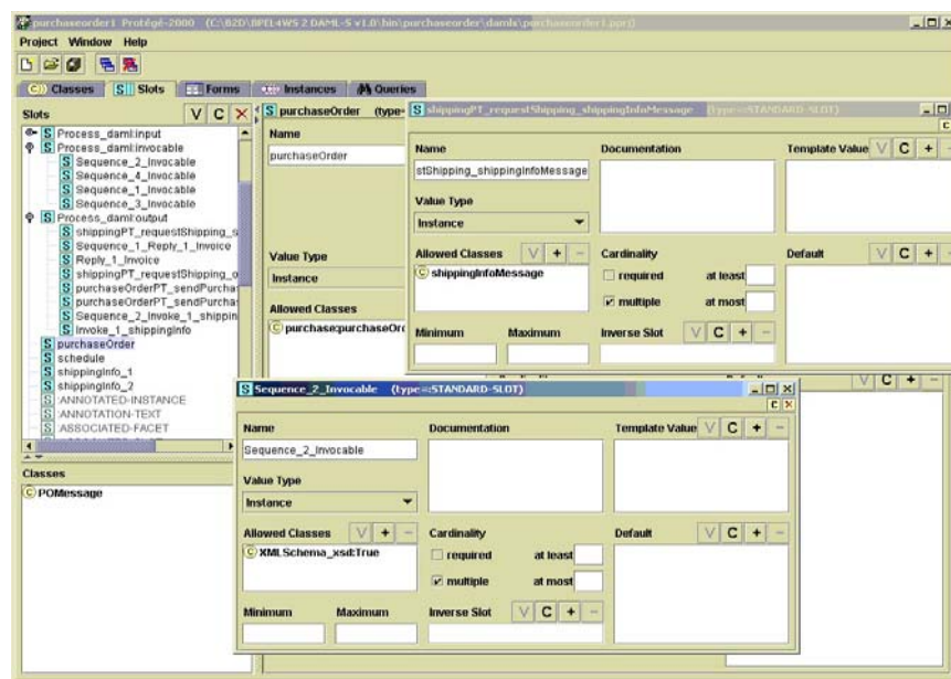
Figure 2: Slots of PurchaseOrder Process
