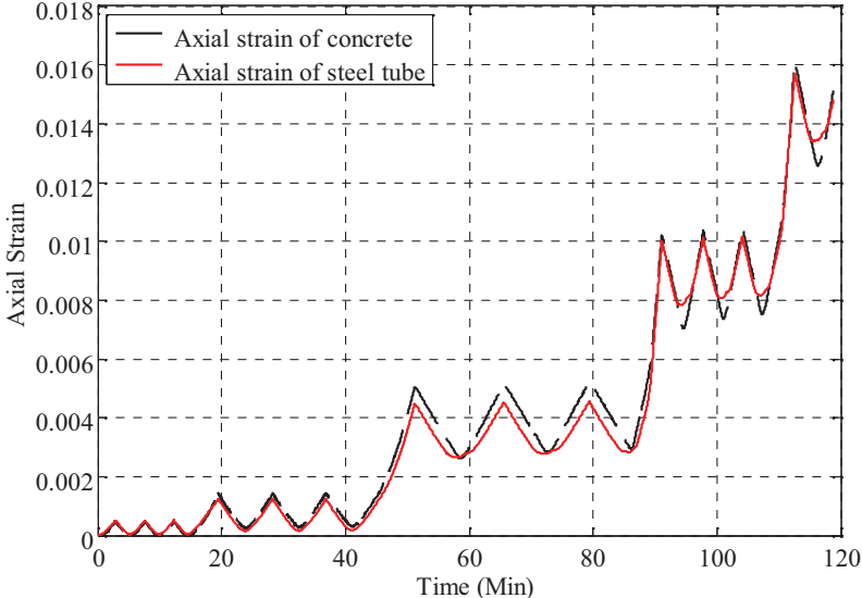
Figure 5. Axial strains of concrete and steel tube.
