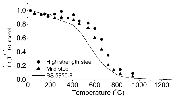
Fig. 6. Comparison of reduction factors of 0.5% strength predicted by BS5950-8 with test results
