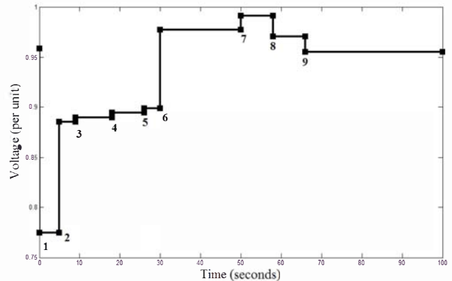
Fig.5. Change in the load voltage in bus 32 by the applied countermeasures.
