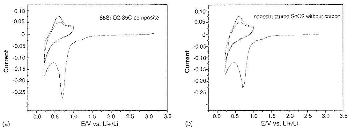
Fig. 5. Cyclic Voltammograms for (a) a nanostructured 65SnO 2 -35C composite electrode and (b) a nanostructured SnO 2 without carbon electrode. Scan rate 0.1 mV s -1 .
