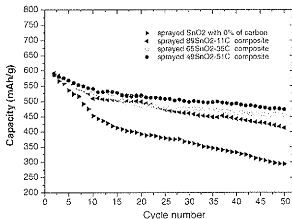
Fig. 6. Discharge capacity vs. cycle number for the potential range from 0.1 to 1.3 V for the nanostructured SnO 2 and SnO 2 -carbon composites.
