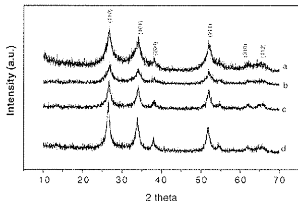
Fig. 2. X-ray powder patterns of sprayed samples: (a) \text{SnO}_2 without carbon and \text{SnO}_2 -carbon composites; (b) 89\text{SnO}_2 \cdot 11\text{C} ; (c) 65\text{SnO}_2 \cdot 35\text{C} ; and (d) 49\text{SnO}_2 \cdot 51\text{C} .
