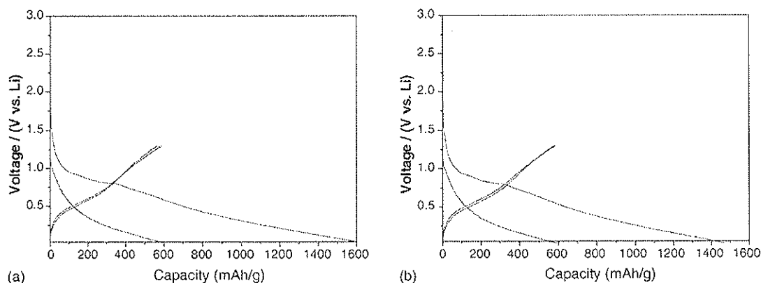
Fig. 4. The first and second discharge and charge curves of (a) nanostructured SnO 2 without carbon and (b) 65SnO 2 -35C composite at 0.04 mA cm -2 .
