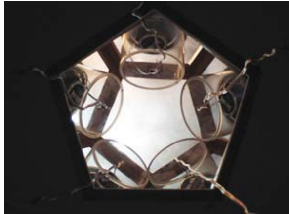
Figure 2 shows five of the ten loudspeakers each positioned in the centre of one of the pentagons on the side of the structure. An image projector is mounted in the plinth and projects through the pentagon at the base of the structure onto the pentagon at the top.
