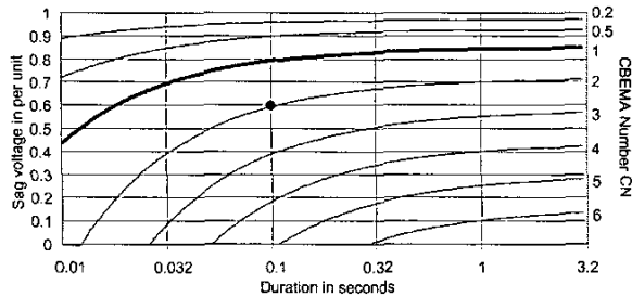
Fig. 1 Sag contours for determining sag severity
