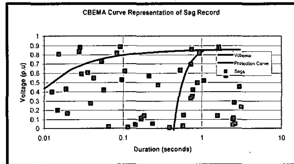
Fig. 3 Sag scattergraph showing CBEMA curve (top left) and Protection curve (right)
