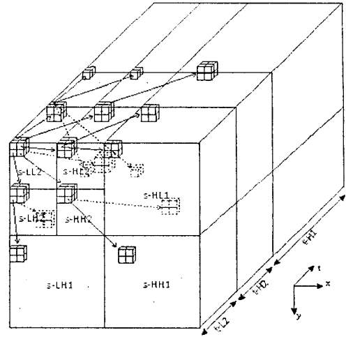
Figure 2. A 3D wavelet decomposition of a GOF with 2 levels of both temporal and spatial decomposition (21 spatiotemporal bands). The parent-offspring relationship between the wavelet coefficients assumed by 3DSPIHT is also shown.
