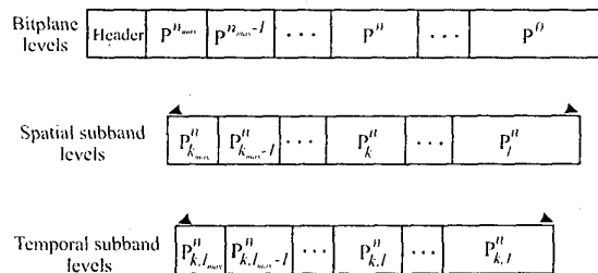
Figure 3. Structure of the FS-3DSPIHT encoder bitstream which is made up of different quality, spatial and temporal resolution parts. P^n_{k,l} denotes the codepart that obtain for coding the spatiotemporal subband set level (k,l) (i.e. B_{k,l} ) at bitplane level n .
