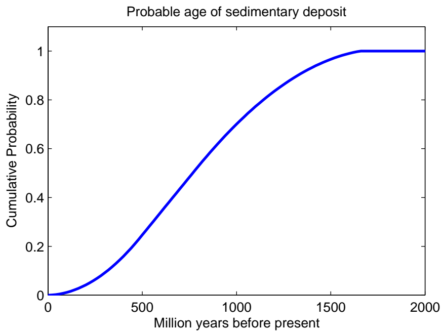
Figure 10: Estimated cumulative distribution for sedimentary deposit age. Calculated from information in figures 8 & 9, and equation (9).
