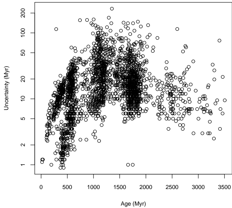
Figure 3: All the zircon ages and their uncertainties.
