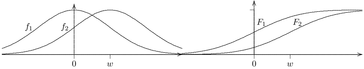
Figure 2: The distributions \mu_1 and \mu_2 showing densities f_1 & f_1 and cumulative distribution functions ( F_1 & F_2 ).
