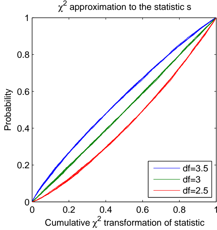
Figure 7: A comparison of the distribution of the statistic s of equation (7) after being transformed using cumulative \chi^2 distributions.
