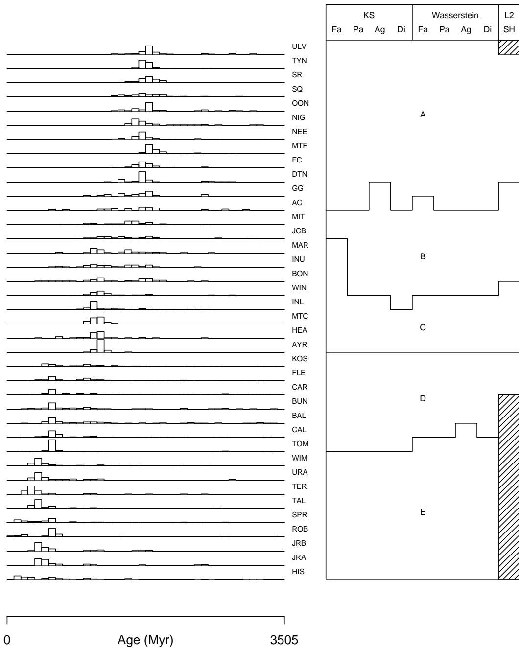
Figure 5: Age distributions of zircons sampled from 38 sites (identified by the codes in the central column, that indicate the location in central and eastern Australia from where the samples came), and classifications into five clusters. The rightmost column shows the results of [5] for 25 of the samples.
