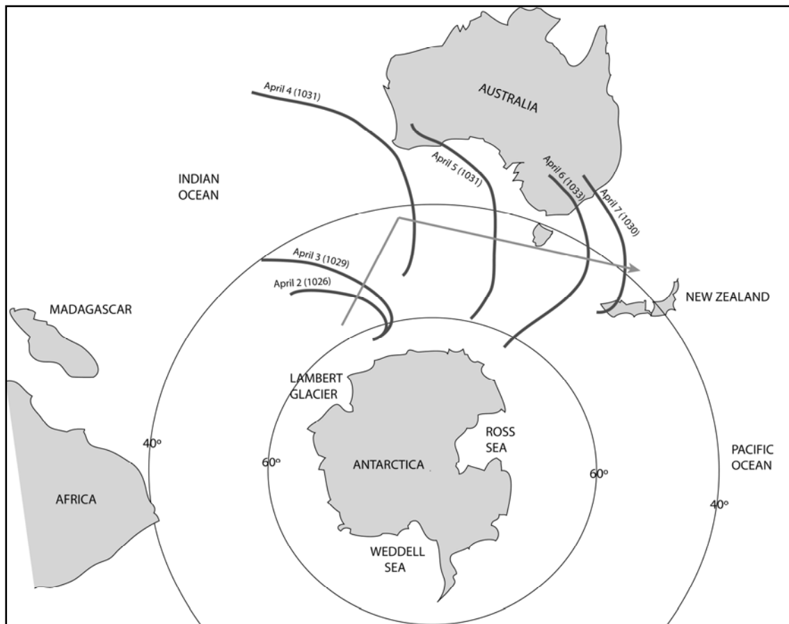
Figure 3: MPH originating from the Lambert Glacier on 2 April 2004. Its pathway is peaked, moving rapidly over Australia and then drifting southward.
