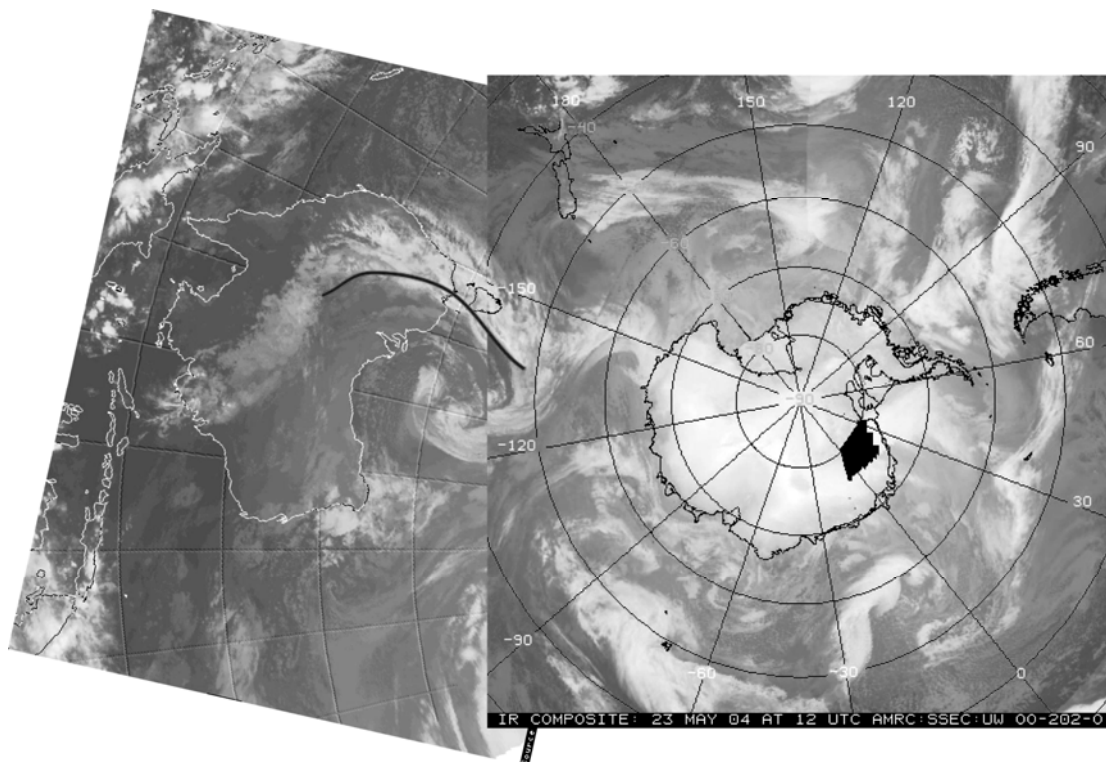
Figure 1: An example of the traced cloudband preceding the arrival of a Mobile Polar High over eastern Australia on 24 May 2004 (Commonwealth Bureau of Meteorology, 2004). Note the pattern of speckled cloud over the Bight, indicative of an infusion of cold air over the continent following the passage of the cloudband.
