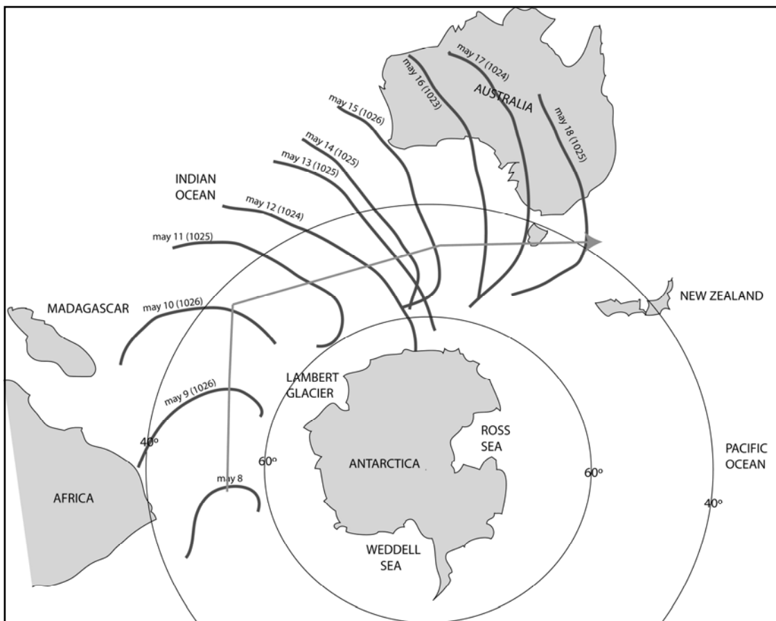
Figure 2: Passage of a MPH originating on 8 May, 2004 from the Weddell Sea. Its pathway is flat showing minimal change in latitude. An additional feature is a northwest cloudband originating in the tropics of the Indian Ocean and moving southeast across Australia.
