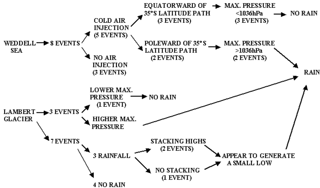
Figure 5: Proposed model of MPH characteristics leading to rainfall production of >50mm in 24hrs in southeastern Australia, 2000 and 2004.
