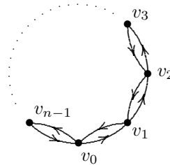
FIGURE 2. The 1-graph D_n
