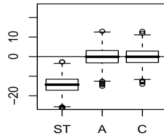
Scenario 2: Unknown lambda, Slope
