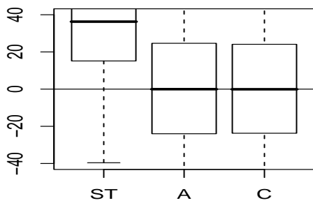
Scenario 2: Unknown lambda, Intercept
