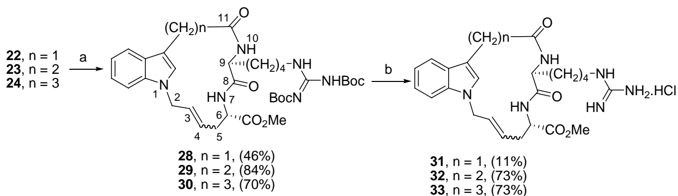
Scheme 3. Reagents: a) N,N' -diBoc- N -triflylguanidine, \text{Et}_3\text{N} , \text{CH}_2\text{Cl}_2 . b) TFA, \text{CH}_2\text{Cl}_2 .
