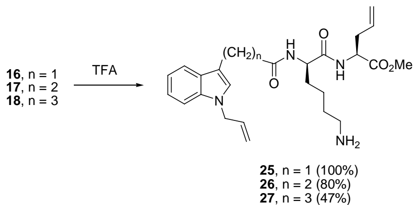
Scheme 2. Deprotection of acyclic indole peptides.
