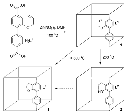
Fig. 1 The structure of H_2L^1 and synthetic conditions to form 1–3 . One network and the major ligand component of each PSR is shown.
