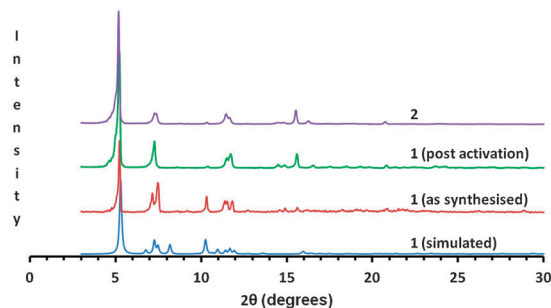
Fig. 4 PXRD patterns for 1 and 2 .
