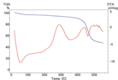
Fig. 3 TG-DTA curves for heating dried 1 to 550 °C. The blue curve shows the TG response. The red curve shows the DTA response.
