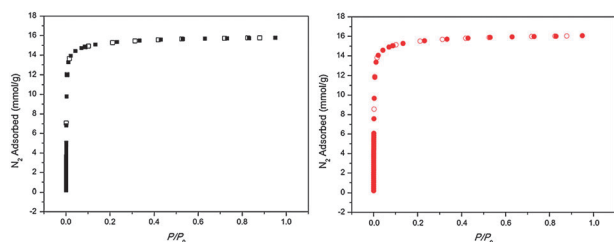
Fig. 5 Nitrogen gas adsorption/desorption isotherms for the in situ conversion of 1 (left) to 2 (right). Closed squares/circles adsorption, open squares/circles desorption.
