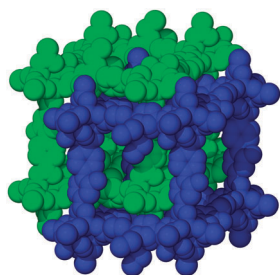
Fig. 2 The doubly interpenetrated structure of 1 .
