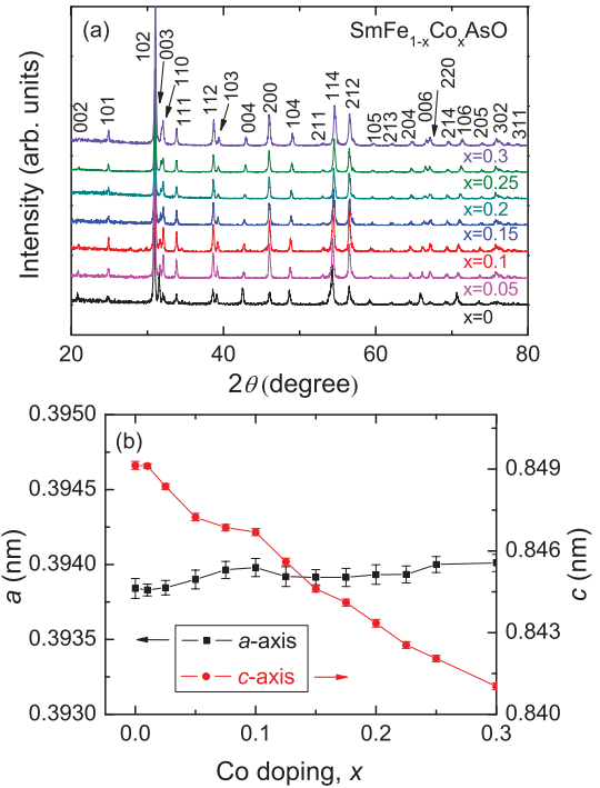
FIG. 7. (Color online) Structural characterization of \text{SmFe}_{1-x}\text{Co}_x\text{AsO} samples. (a) Powder x-ray diffraction patterns of representative \text{SmFe}_{1-x}\text{Co}_x\text{AsO} samples. (b) Lattice parameters as a function of Co content.
