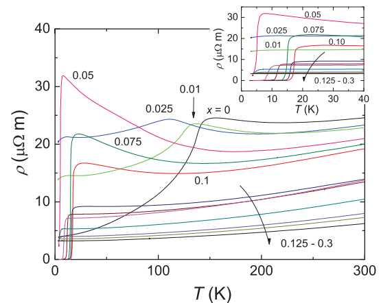
FIG. 8. (Color online) Temperature dependence of resistivity ( \rho ) for the \text{SmFe}_{1-x}\text{Co}_x\text{AsO} samples. Inset: the enlarged plot of \rho versus T for low temperatures, showing the superconducting transitions.
