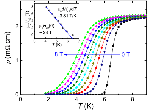
FIG. 5. (Color online) SC transitions in resistivity under magnetic fields ( \mu_0 H=0, 1, 2, 3, 4, 5, 6, 7 , and 8 T) for \text{LaFe}_{0.96}\text{Ni}_{0.04}\text{AsO} sample. The inset shows the upper critical fields as a function of temperature.
