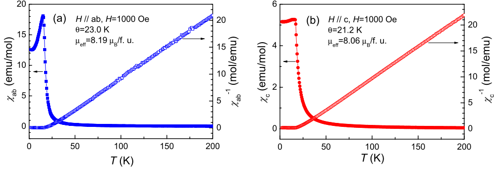
FIG. 6. (Color online) Temperature dependence of magnetic susceptibility for Eu(Fe 0.89 Co 0.11 ) 2 As 2 . The measurements were performed in field cooling mode under the applied field of 1000 Oe. (a) H \parallel ab ; (b) H \parallel c .
