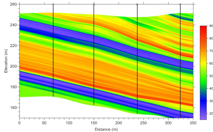
Figure 6 - The GSR model for the same section as Figure 5. Again the layer boundaries of Figure 4 have been used to guide the interpolation of the GSR data between holes.
