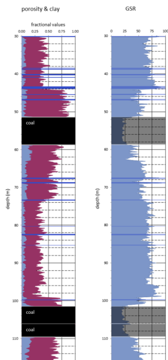
Figure 2 - Interpretation of the geophysical logs from Figure 1. On the left, the porosity is shown in blue and the clay content is shown in red. The clay content is lower in the sandstone than in the siltstone. GSR values are higher in the sandstone than in the siltstone.
