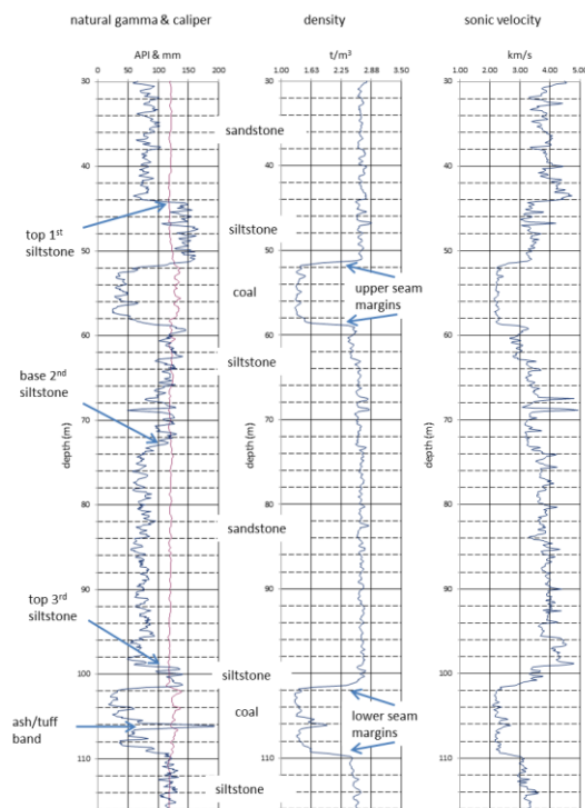
Figure 1 - Example of geophysical logs obtained from an exploration borehole. These logs allow identification of the major rock types present - coal, sandstone and siltstone. A tuff band is also present in the lower coal seam.
