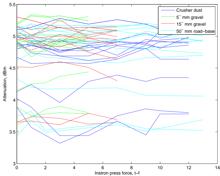
Figure 5 - Cable attenuation versus Instron press force for different sample materials
