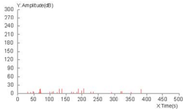
Figure 3 - Changes in EMR amplitude with time (Channel 1 is located in copper shielding net)
