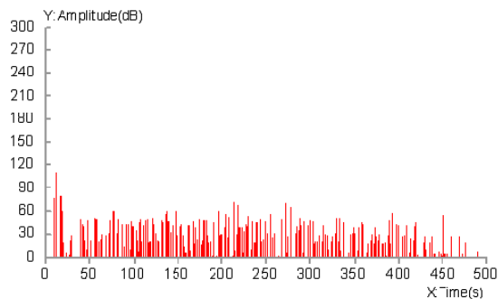
Figure 4 - Changes in EMR amplitude with time (Channel 5 is located in outer of copper shielding net)
