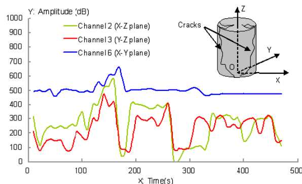
Figure 10 - EMR fitted curves from circle antenna (Channel 6) and line antenna (Channel 2 and 3)
