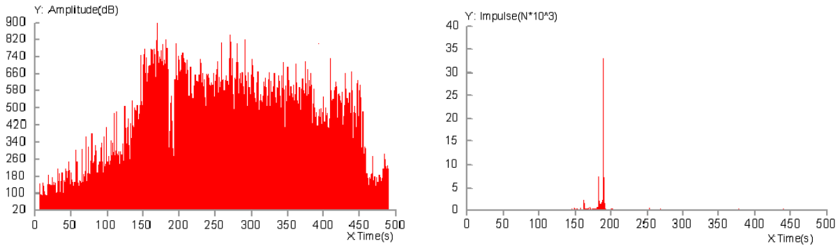
Figure 6 - Changes in AE amplitude and impulse with time (Channel 7-150 kHz)
