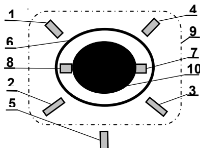
1, 2, 3, 4 and 5-line type EMR antenna; 6-circle EMR antenna; 7 and 8-AE sensor; 9-copper shielding net; 10-sample
