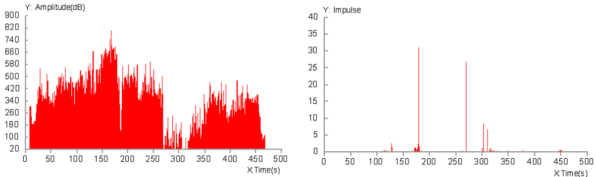
Figure 7 - Changes in EMR amplitude and impulse with time (Channel 2-150 kHz)
