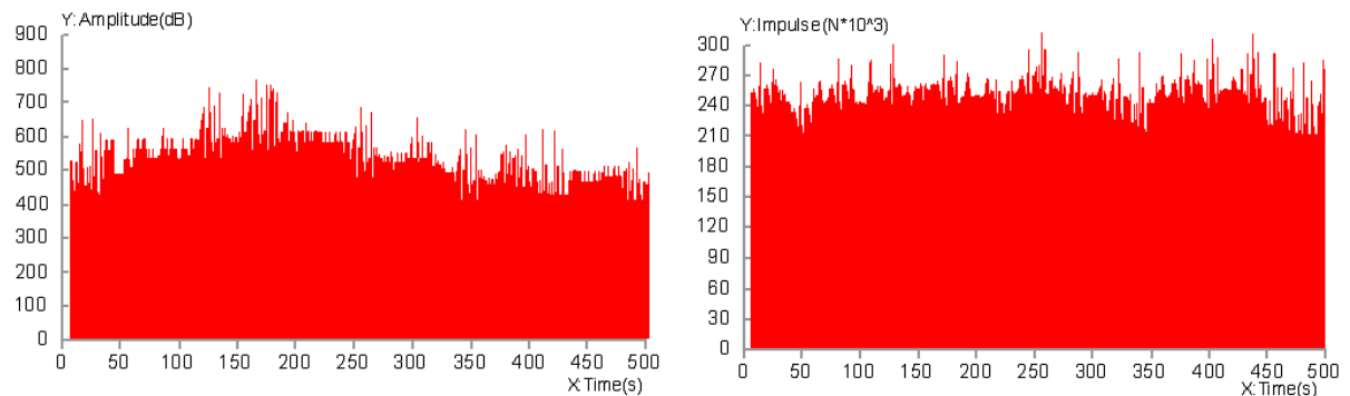
Figure 9 - Changes in EMR amplitude and impulse with time (Channel 6: circle antenna-broadband)
