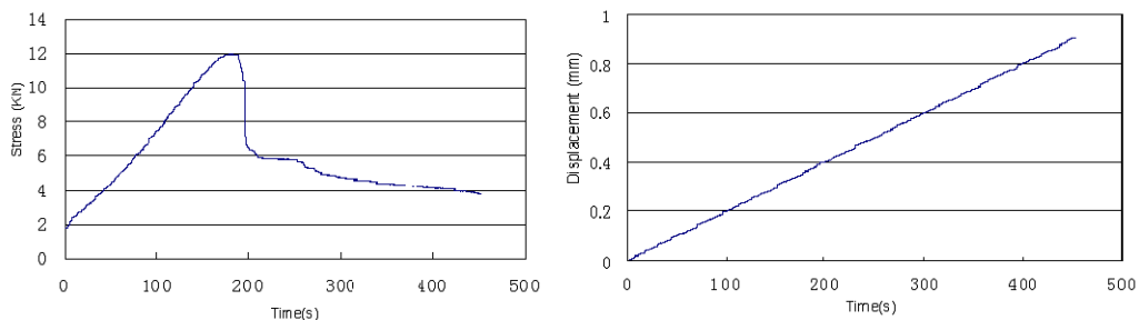
Figure 5 - Changes in stress and displacement with time
