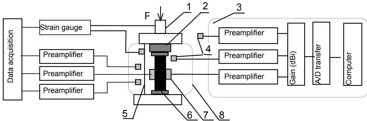
1-Pressure plateau; 2-Stress sensor; 3-Data acquisition system; 4-Line type EMR antenna; 5-Displacement sensor; 6-Insulating paper; 7-Acoustic emission sensor; 8-Copper shielding net
