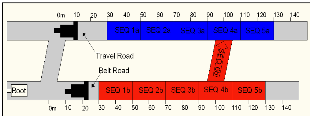
Figure 5 - Super panel sequence plan
