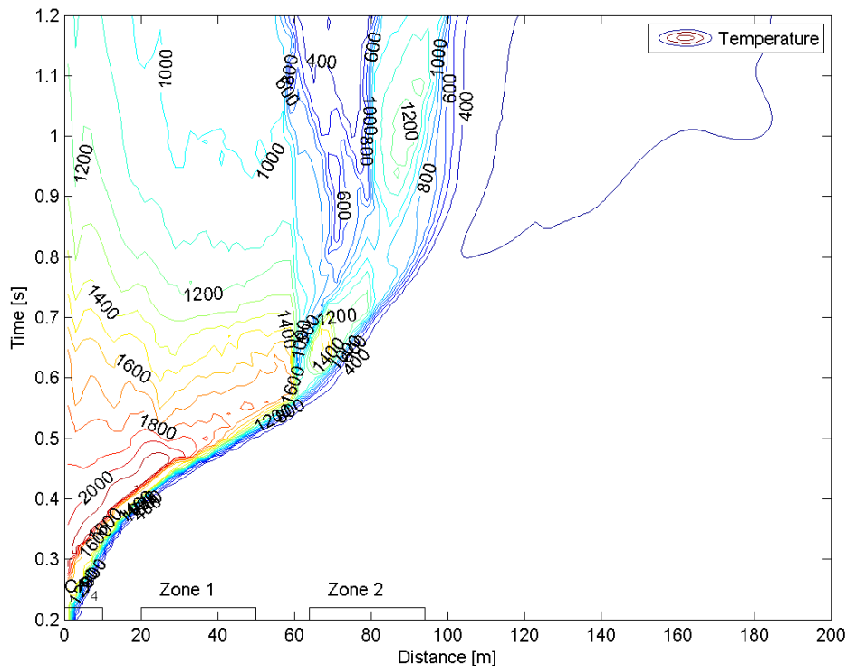
Figure 9 - Triple ring, 100 \mu\text{m} droplets, 200 l/s flowrate
