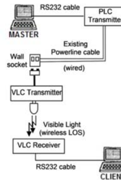
Figure 1: System Design
