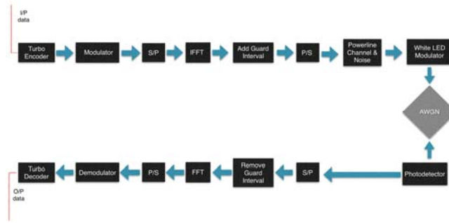
Figure 2: Integrated system block diagram
