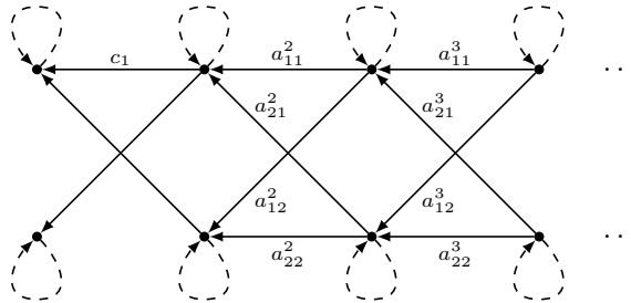
FIGURE 2. The crossed-produce 2-graph of Example 3.3(2)
