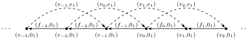
FIGURE 1. The crossed-produce 2-graph of Example 3.3(1)
