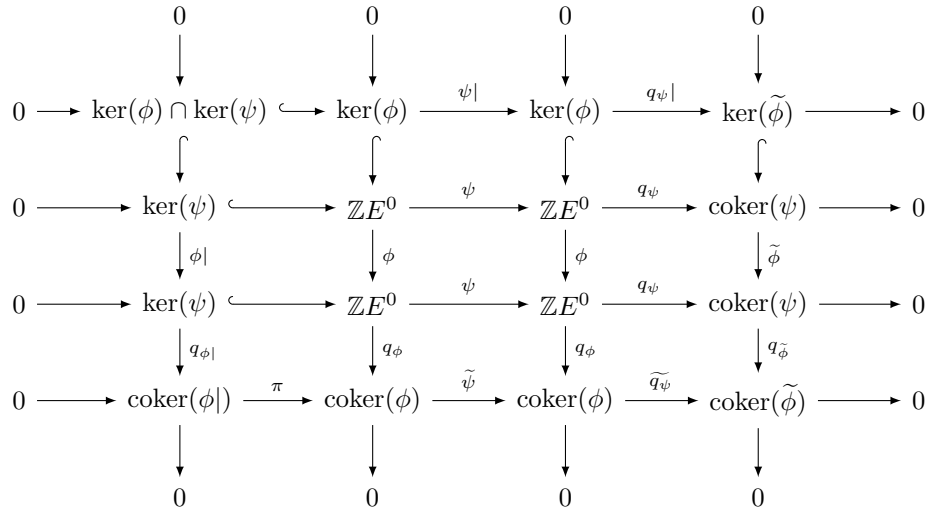
FIGURE 3. The 16-term diagram for \phi and \psi .
