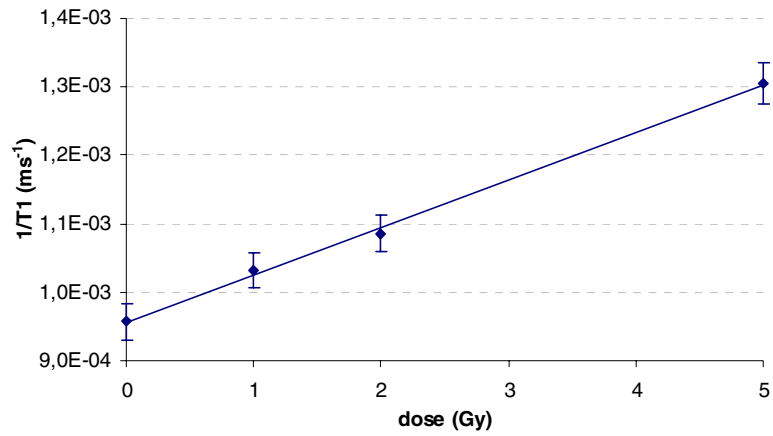
Figure 2. Dose response curve of the Fricke gel irradiated by a monoenergetic beam of 78.8 keV. The error bars represent the standard deviation of the 1/T1 values observed on the NMR image within the calibration tubes.
