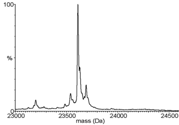
Figure 2. ESI-MS spectrum of purified \alpha_{S1} -casein with a major peak occurring at 23, 619 kDa corresponding to \alpha_{S1} B-casein 8P. Reprinted with permission from [17]. Copyright (2011) Elsevier Inc.
