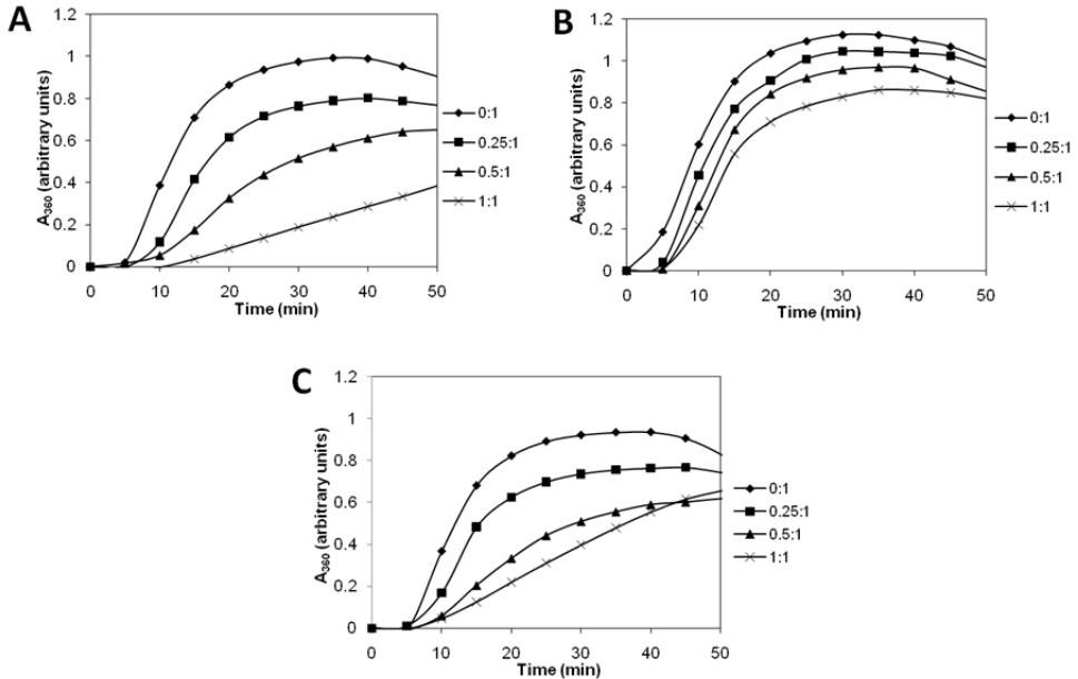
Figure 8. Chaperone activity of A) \alpha_{S1} -, B) \alpha_{S1} - and C) \alpha_{S2} -casein against amorphously aggregating catalase, in the presence of 0.1 M NaCl and various w:w ratios as determined by light scattering at 360 nm. The 0:1 ratio in each assay represents catalase aggregation in the absence of \alpha -casein i.e. no chaperone present. Reprinted with permission from [17]. Copyright (2011) Elsevier Inc.
