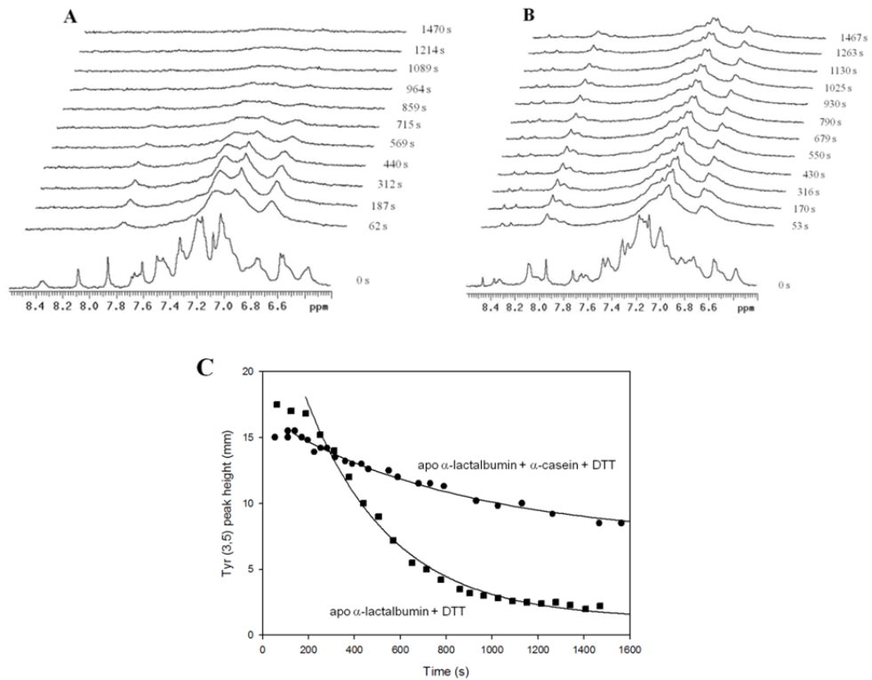
Figure 5. Real-time 1 H NMR spectroscopy of apo- \alpha -lactalbumin under reduction stress at 37°C in the presence and absence of \alpha s-casein. Stacked plots of 1D 1 H NMR spectra show molten globule formation by reduced apo- \alpha -lactalbumin in A) the absence and B) the presence of \alpha s-casein at a 2:1 (w:w) ratio. First-order decay of the resonance arising from the tyrosine (3,5) ring protons at 3.5 ppm in both cases (C) was used to calculate rates i.e. peak height (mm) v time (s). Reprinted with permission from [18]. Copyright (2005) American Chemical Society.
