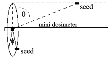
Fig. 1. Azimuthal isotropy measurement geometry (solid lines) and polar angle measurement geometry (dotted lines), where \phi is the azimuthal angle about the minidosimeter axis and \theta is the polar angle. The horizontal dotted line represents the location of the catheter within which the seed position was varied for the polar angle measurements.
