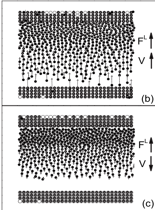
FIG. 2. (a) A numerical clockwise V_x - F^L loop. The arrows indicate the evolution of the driving force. The inset displays the time evolution of the average velocity of vortices. It is noted that negative velocity occurs when the driving force is decreasing and small. (b) Vortex trajectories [from beginning ( \bullet ) to end ( \Delta )] for driving forces from F^L = F_B + 0.26f_0 to F^L = F_B in the descending branch. The vortices are moving in the same direction as the driving force. The open circles are pinning centers. (c) Vortex trajectories [from beginning ( \bullet ) to end ( \nabla )] for driving forces from F^L = F_B to F^L = F_B - 0.26f_0 in the descending branch. In this case, due to the fact that the repelling forces from the captured vortices by strong pinning are larger than F^L , the vortices in weak pinning region are drifting in the opposite direction of the driving force and return to their equilibrium positions. We have used f_{pv0} = 30f_0 , dF^L/dt = 0.01f_0/t_0 , and d/L = 4/30 .
