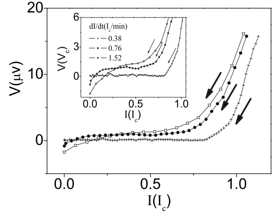
FIG. 6. Experimental V-I curves upon descending current (the ascending branches are not shown here for clarity) for different dI/dt and at temperature T=77 \text{ K} and reduced field H/H_{c2}=8.33 \times 10^{-3} . It is seen that negative voltage occurs for higher CSR, which is in good agreement with the numerical results shown in Fig. 3. The inset shows the enlarged view of the V-I curves. I_c = 13 \text{ A} which is the typical critical current at lower CSR for our samples, and the voltage criterion is V_c = 1 \mu\text{V} . H_{c2}(T=77 \text{ K}) = 0.6 \text{ T} for field parallel to the c axis of Ag/Bi-2223 polycrystal tape (Ref. 21).
