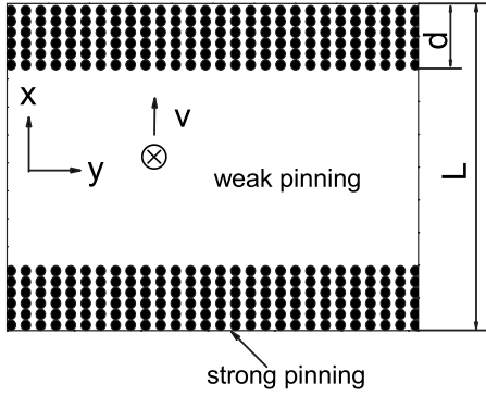
FIG. 1. Sketch of the xy section of the simulation box at z=0 . The black spots and empty squares denote the strong and weak pinning centers, respectively. The Lorentz force is in the x direction, and magnetic field is in the z direction.
