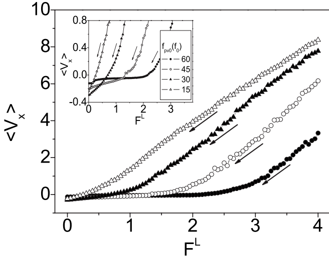
FIG. 5. Effect of the inhomogeneity of pinning strength f_{pv0} on ANM and size of the hysteresis loop. d/L=6/30 and dF^L/dt=0.1f_0/t_0 . The inset shows the magnification of the V-F^L curve for low F^L . It is noted that ANM and the loop become too small to observe for very small f_{pv0} .
