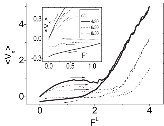
FIG. 4. Effect of d/L on the apparent negative motion. The larger d/L means that there are fewer vortices in the weak pinning region and they will only make a shorter reversal journey before reaching their equilibrium positions (thus having a shorter relaxation time). Therefore, the larger d/L is, the smaller the ANM (also the hysteretic V - F^L loop) is. f_{pv0} = 60f_0 and dF^L/dt = 0.1f_0/t_0 . The inset shows the magnification of the V - F^L curve for low F^L .
