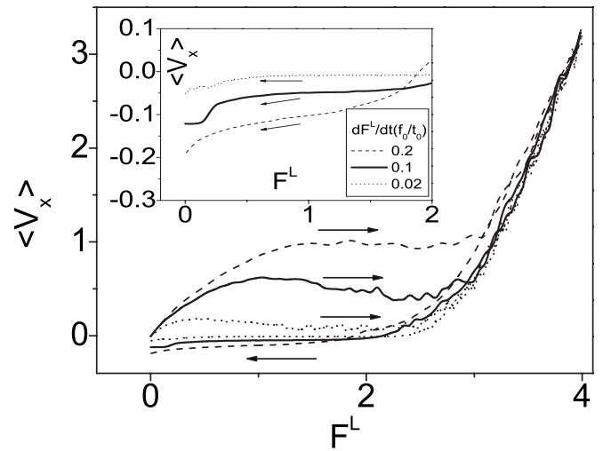
FIG. 3. Effect of driving force scanning rate on the apparent negative motion (with f_{pv0} = 60f_0 , d/L = 6/30 ). The inset shows the magnification of the descending branch of V - F^L loop for low F^L . ANM and hysteresis loop become invisible with the decreasing scanning rate. It is clear that the negative motion and the hysteresis loop are more apparent at fast scanning rate than at slow rate.
