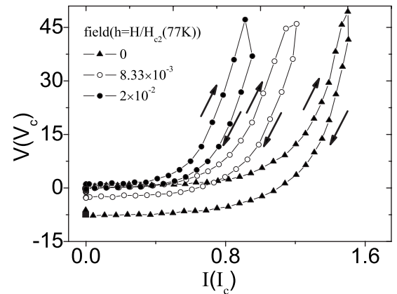
FIG. 7. Experimental V-I curves at different reduced fields. The ANM and the size of hysteretic V-I loops decrease with field. T = 77 \text{ K} and dI/dt=9.22(I_c/\text{min}) .
