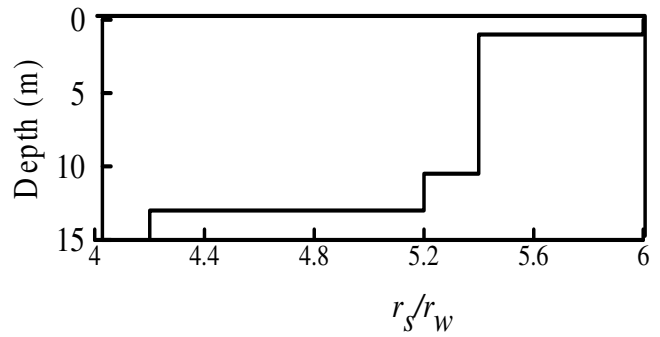
Figure 13: Variation of smear zone with depth by the Cavity Expansion theory (where, r_s : radius of smear zone, and r_w : radius of drain)
