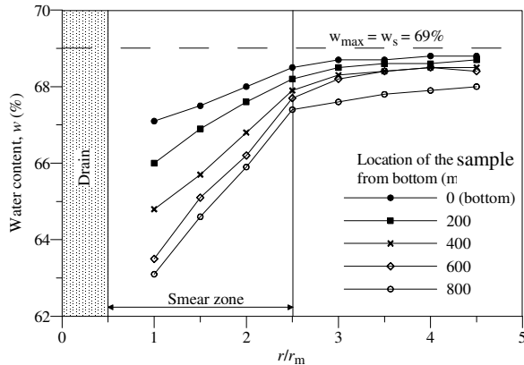
Figure 9: Variation of water content with depth and radial distance for an applied pressure of 200 kPa (after Sathanathan and Indraratna, 2006)
