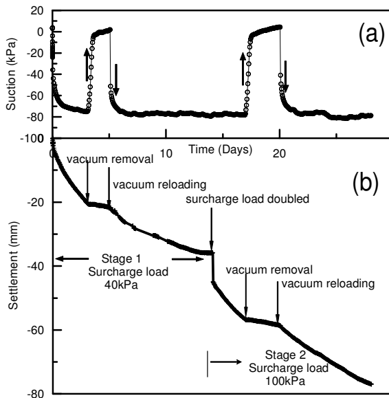
Figure 10: a) Suction in the drain (240mm from bottom) and b) surface settlement associated with simulated vacuum loading and removal (Indraratna et al. 2004)
