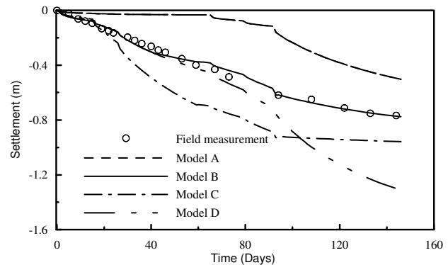
15m Figure 19: Surface settlement time curves of embankment TV1 (modified after Indraratna et al., 2005f)
