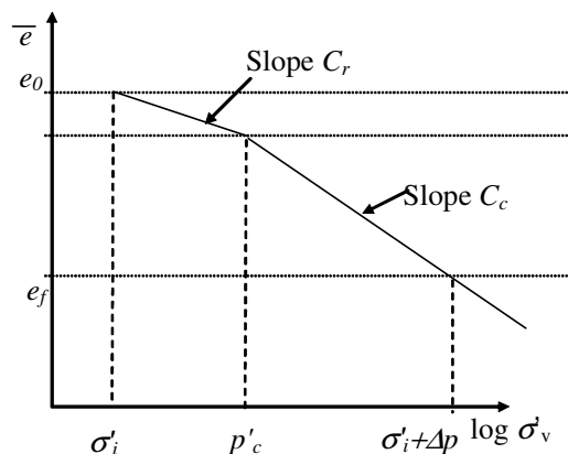
Figure 2: Soil compression curve (after Indraratna et al., 2005b)
