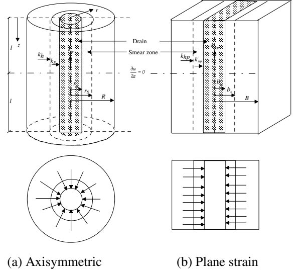
Figure 5: Conversion of an axisymmetric unit cell into plane strain condition (after Indraratna and Redana, 2000)
