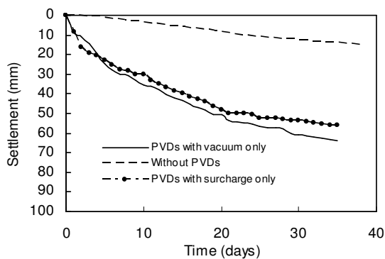
Figure 7. Pre-consolidation settlements
